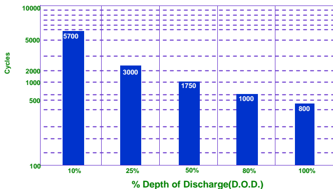
Gel Cycle Life vs Depth of Discharge at +25°C (77°F)* Based on IEC 896-2
