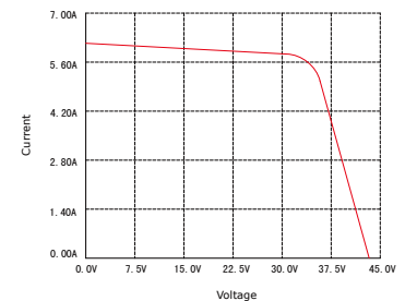
Module IV Graph 190W
